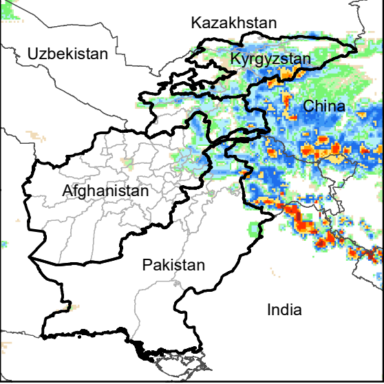
Daily Rainfall estimate for 1 May., 2004
