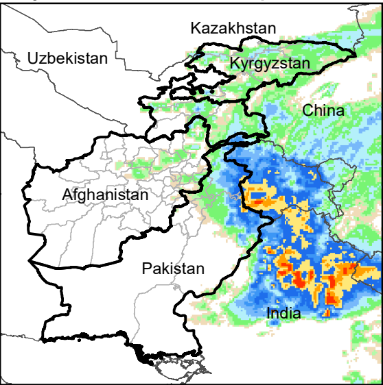
Daily Rainfall estimate for 3 May., 2004
