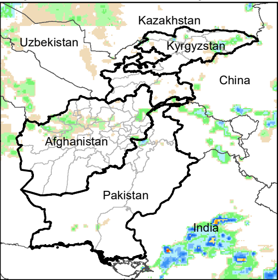
Daily Rainfall estimate for 16 May., 2004
