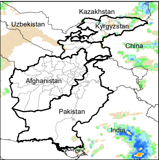
Daily Rainfall estimate for 15 May., 2004
