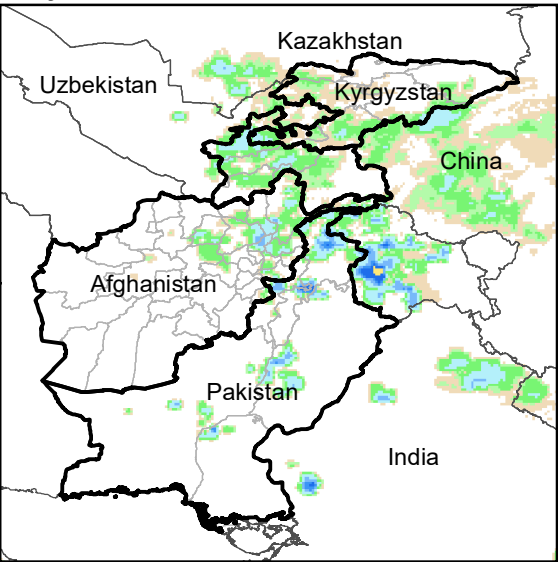
Daily Rainfall estimate for 4 Jun., 2004
