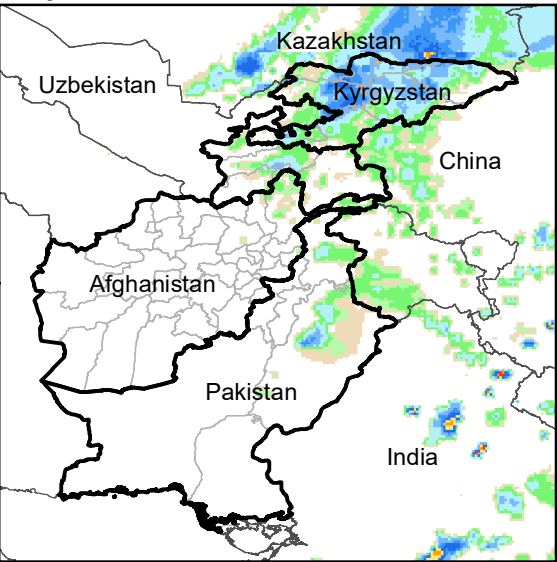
Daily Rainfall estimate for 9 Jun., 2004
