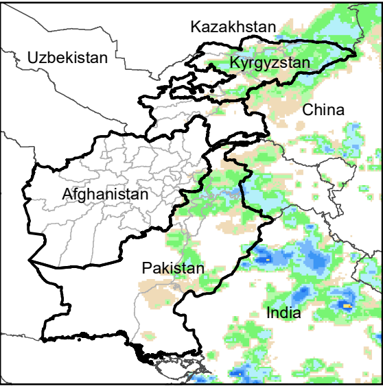
Daily Rainfall estimate for 8 Jun., 2004
