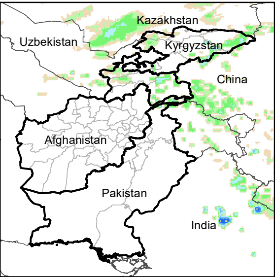
Daily Rainfall estimate for 7 Jun., 2004
