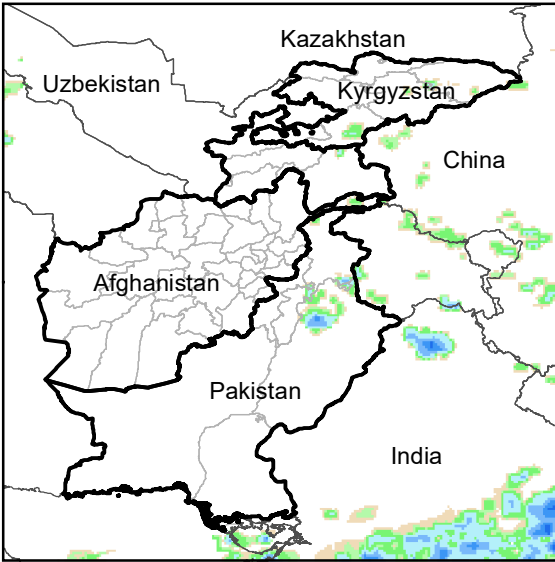
Daily Rainfall estimate for 11 Jun., 2004
