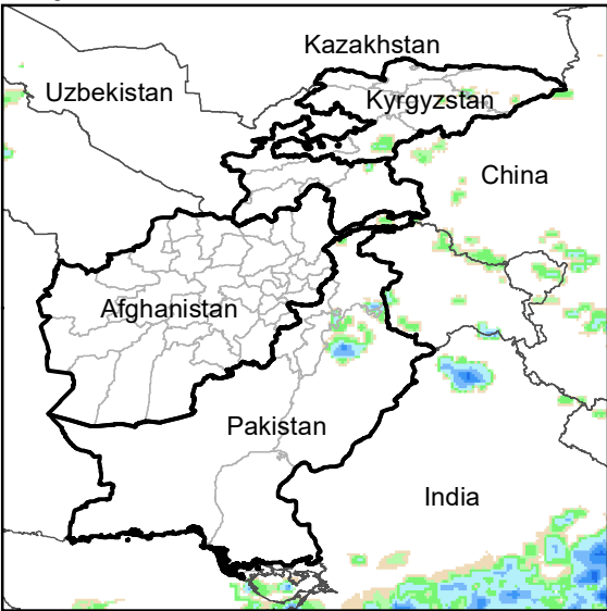
Daily Rainfall estimate for 14 Jun., 2004
