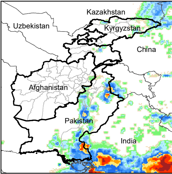
Daily Rainfall estimate for 15 Jun., 2004
