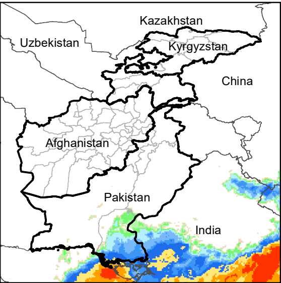
Daily Rainfall estimate for 19 Jun., 2004
