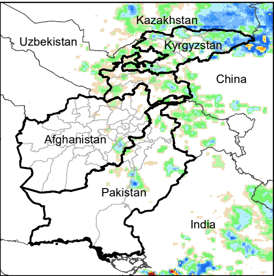
Daily Rainfall estimate for 22 Jul., 2004
