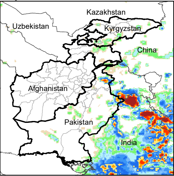
Daily Rainfall estimate for 27 Jul., 2004
