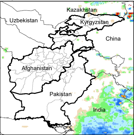
Daily Rainfall estimate for 28 Jul., 2004
