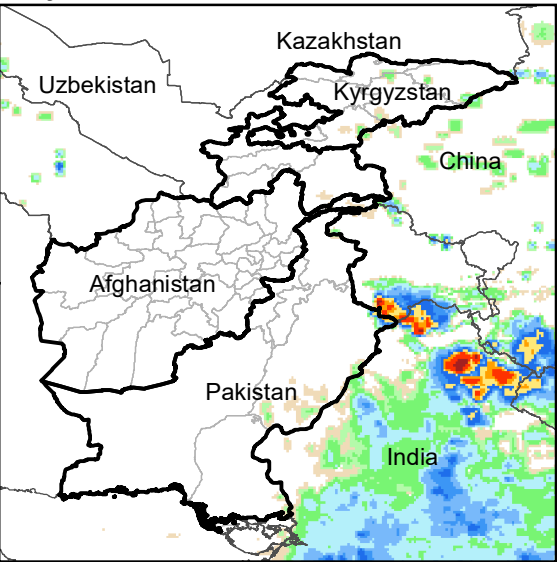
Daily Rainfall estimate for 29 Jul., 2004
