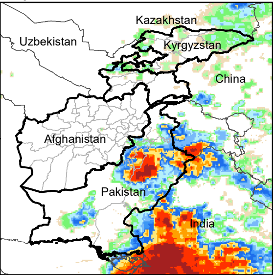
Daily Rainfall estimate for 2 Aug., 2004
