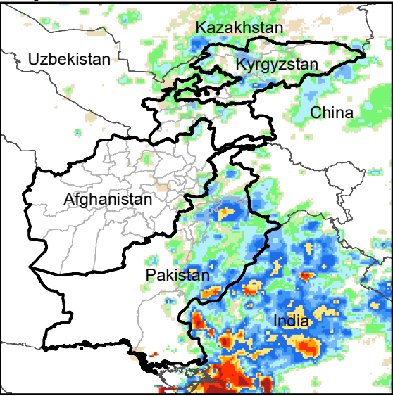
Daily Rainfall estimate for 1 Aug., 2004
