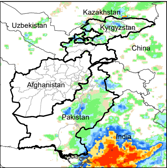
Daily Rainfall estimate for 3 Aug., 2004
