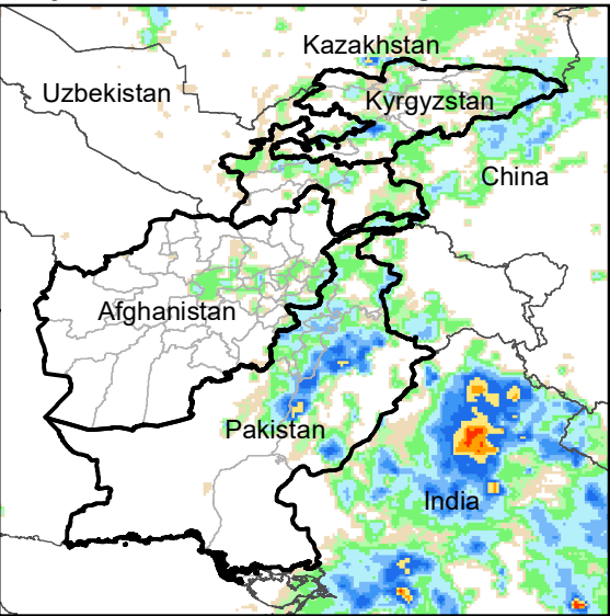
Daily Rainfall estimate for 5 Aug., 2004
