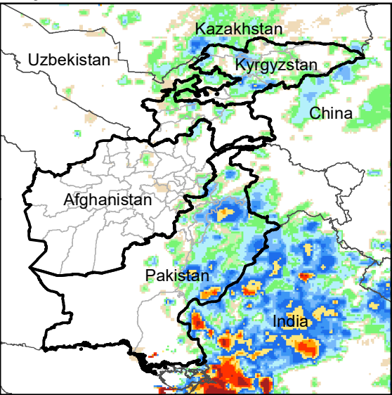
Daily Rainfall estimate for 4 Aug., 2004
