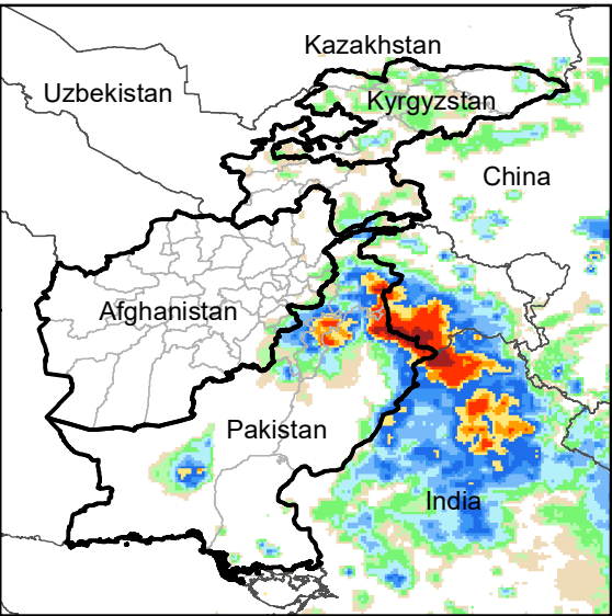
Daily Rainfall estimate for 20 Aug., 2004
