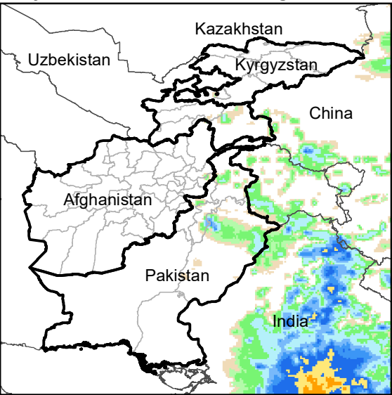
Daily Rainfall estimate for 25 Aug., 2004
