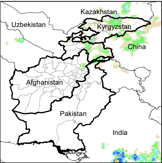
Daily Rainfall estimate for 7 Sep., 2004
