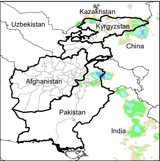
Daily Rainfall estimate for 18 Sep., 2004
