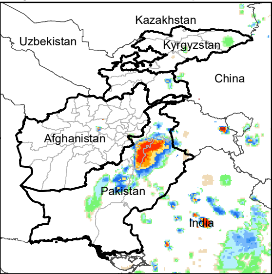
Daily Rainfall estimate for 19 Sep., 2004
