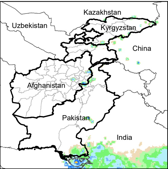
Daily Rainfall estimate for 28 Sep., 2004
