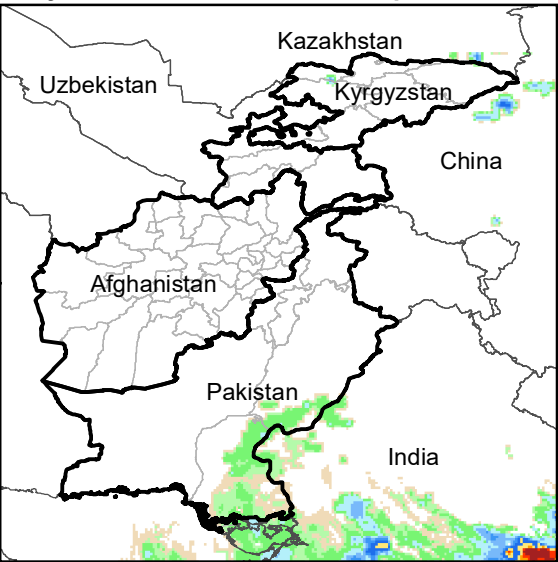
Daily Rainfall estimate for 29 Sep., 2004
