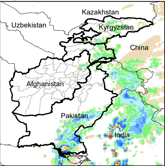
Daily Rainfall estimate for 6 Oct., 2004
