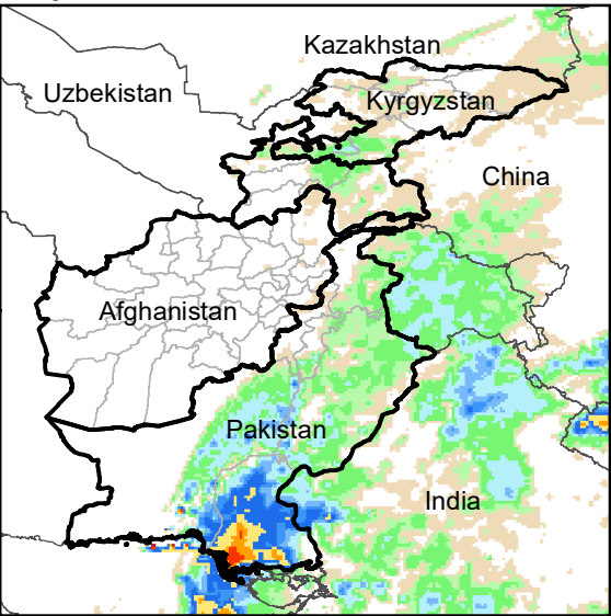
Daily Rainfall estimate for 5 Oct., 2004
