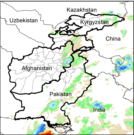
Daily Rainfall estimate for 4 Oct., 2004
