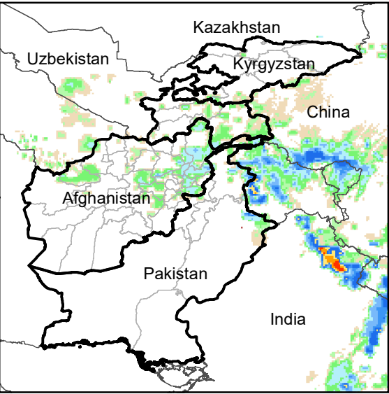
Daily Rainfall estimate for 12 Oct., 2004
