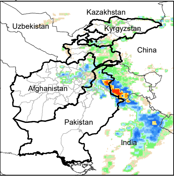
Daily Rainfall estimate for 10 Oct., 2004
