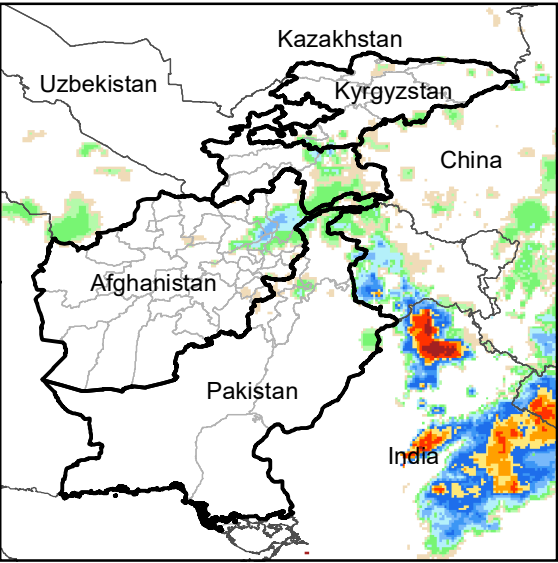
Daily Rainfall estimate for 11 Oct., 2004
