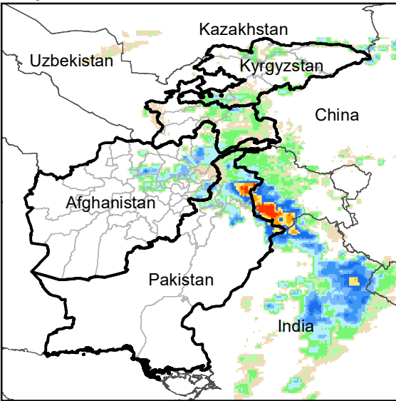
Daily Rainfall estimate for 13 Oct., 2004
