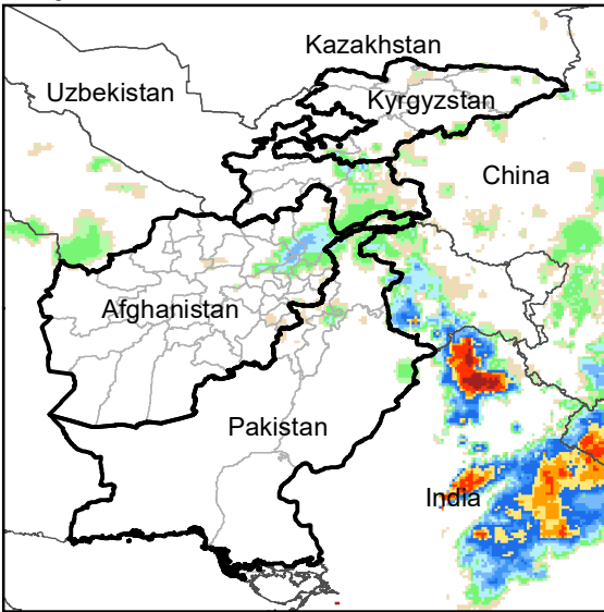
Daily Rainfall estimate for 14 Oct., 2004
