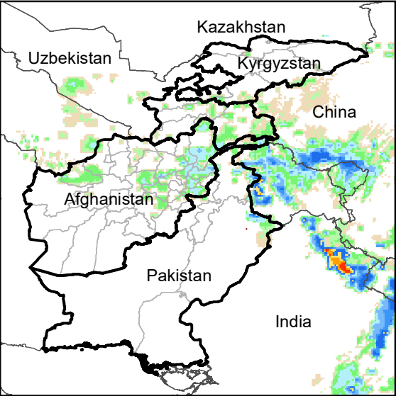
Daily Rainfall estimate for 15 Oct., 2004
