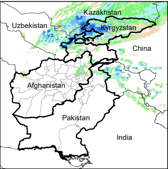
Daily Rainfall estimate for 18 Oct., 2004
