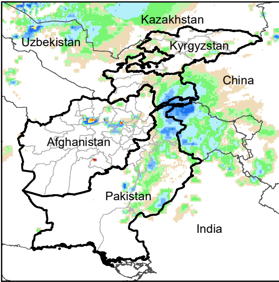
Daily Rainfall estimate for 26 Oct., 2004
