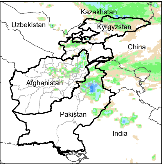
Daily Rainfall estimate for 31 Oct., 2004
