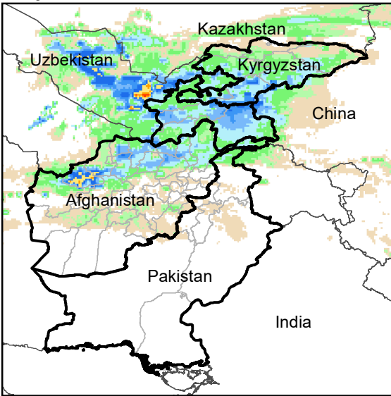
Daily Rainfall estimate for 23 Nov., 2004
