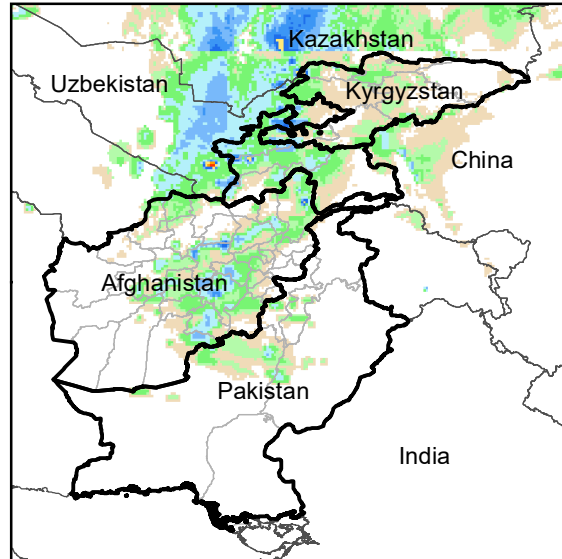
Daily Rainfall estimate for 25 Nov., 2004
