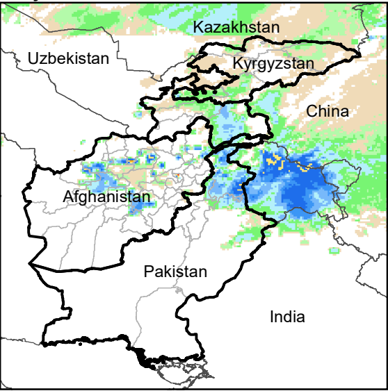
Daily Rainfall estimate for 30 Nov., 2004
