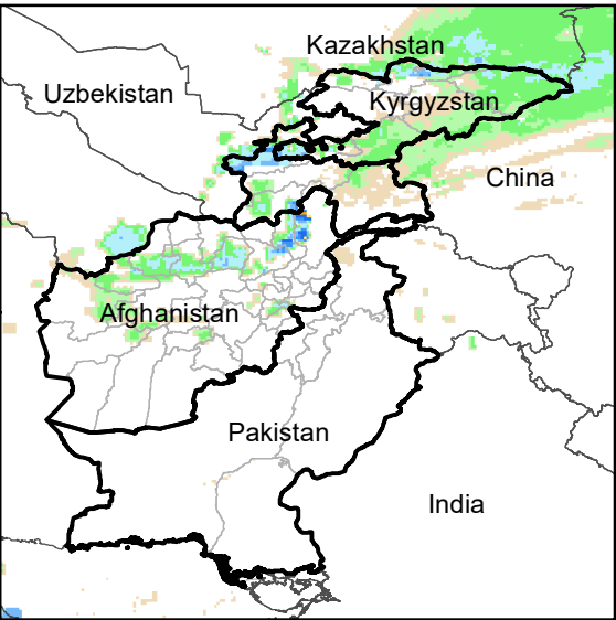
Daily Rainfall estimate for 7 Dec., 2004
