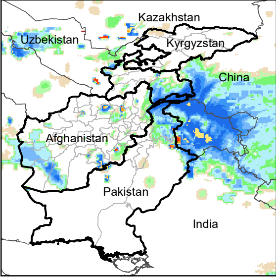
Daily Rainfall estimate for 22 Jan., 2005
