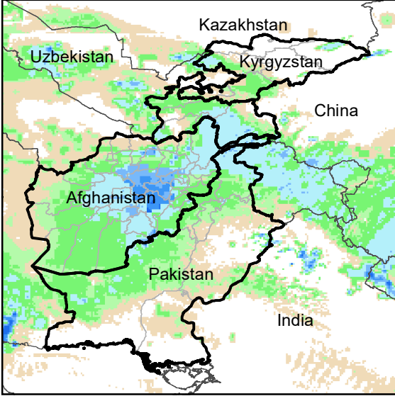
Daily Rainfall estimate for 23 Jan., 2005
