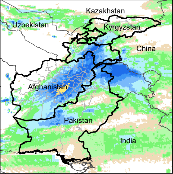
Daily Rainfall estimate for 21 Jan., 2005
