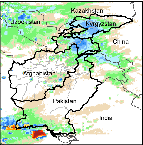
Daily Rainfall estimate for 27 Jan., 2005
