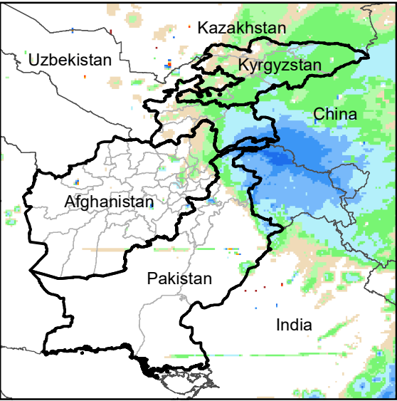
Daily Rainfall estimate for 28 Jan., 2005
