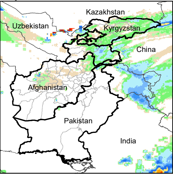
Daily Rainfall estimate for 30 Jan., 2005
