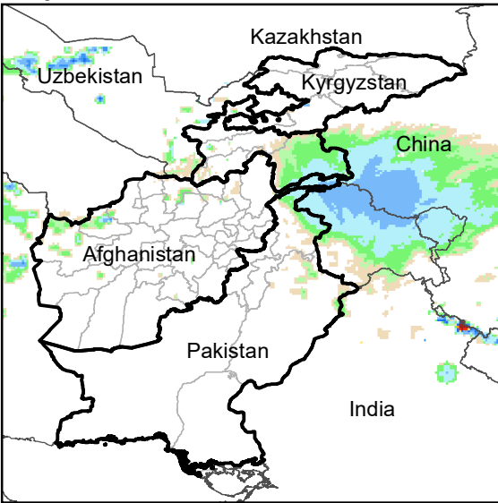
Daily Rainfall estimate for 21 Feb., 2005
