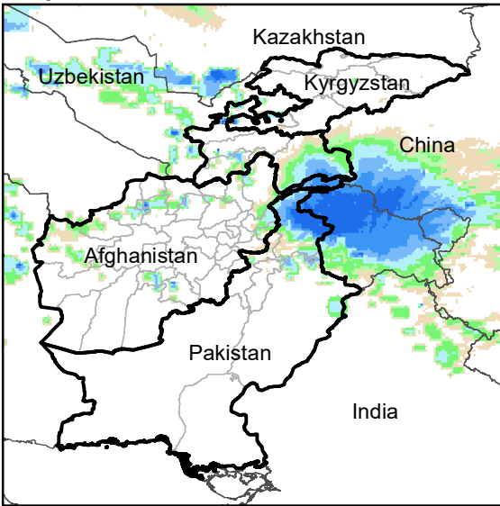
Daily Rainfall estimate for 22 Feb., 2005
