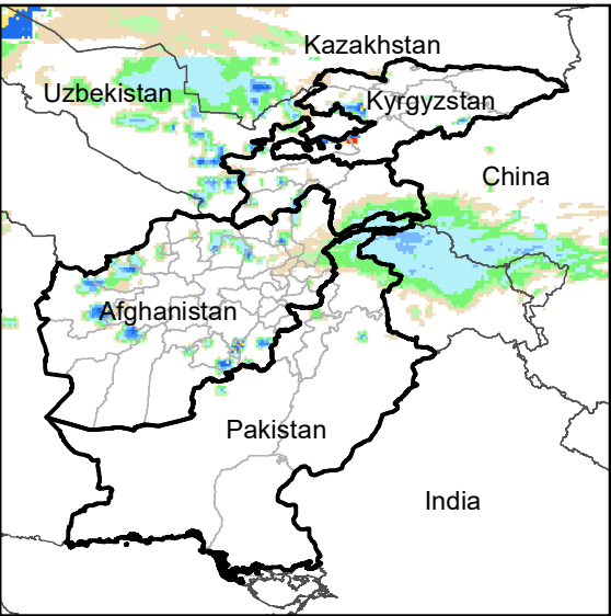
Daily Rainfall estimate for 23 Feb., 2005
