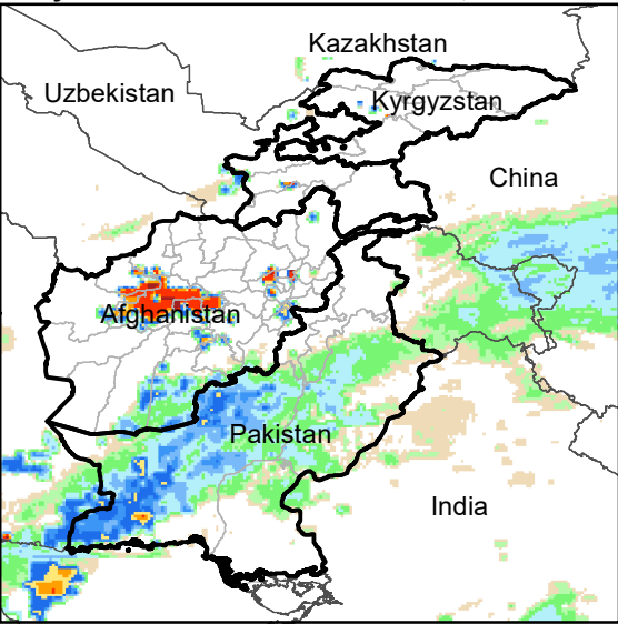
Daily Rainfall estimate for 28 Feb., 2005
