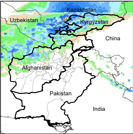
Daily Rainfall estimate for 16 Mar., 2005
