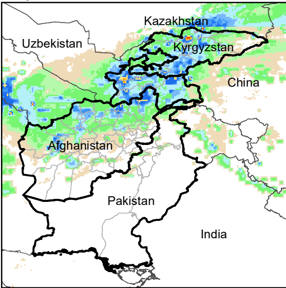
Daily Rainfall estimate for 17 Mar., 2005
