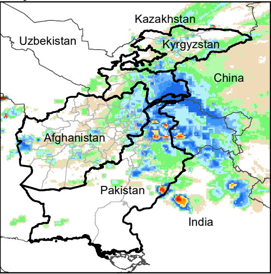
Daily Rainfall estimate for 19 Mar., 2005
