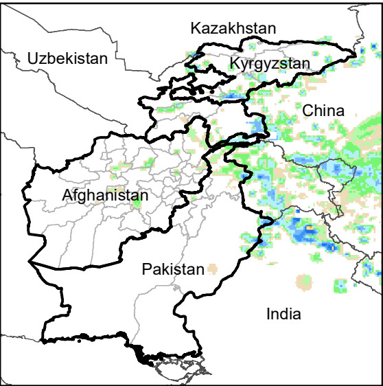
Daily Rainfall estimate for 25 Mar., 2005
