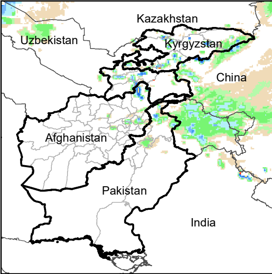
Daily Rainfall estimate for 1 Apr., 2005
