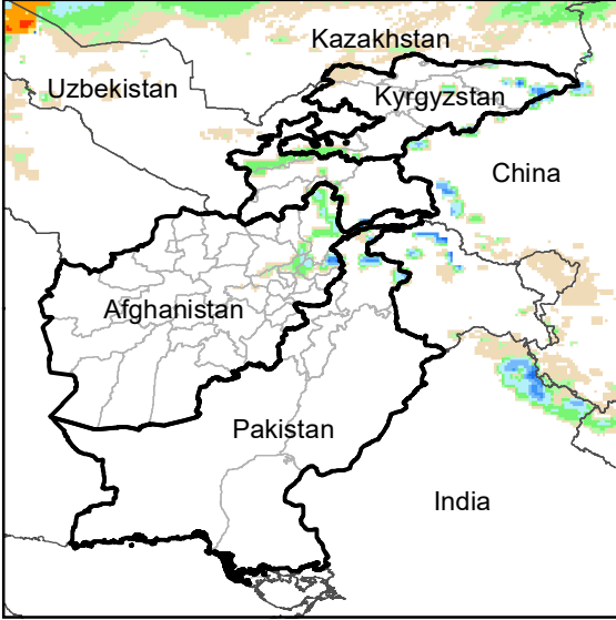
Daily Rainfall estimate for 2 Apr., 2005
