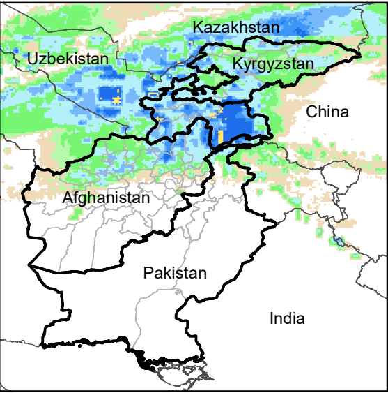
Daily Rainfall estimate for 4 Apr., 2005
