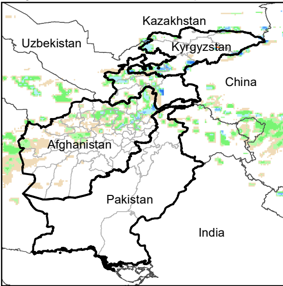
Daily Rainfall estimate for 14 Apr., 2005
