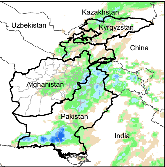
Daily Rainfall estimate for 27 Apr., 2005
