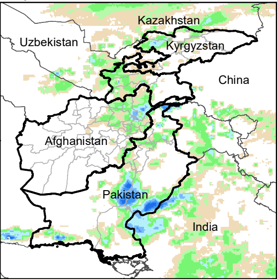
Daily Rainfall estimate for 26 Apr., 2005
