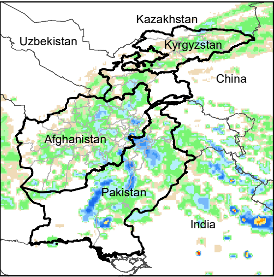
Daily Rainfall estimate for 2 May., 2005
