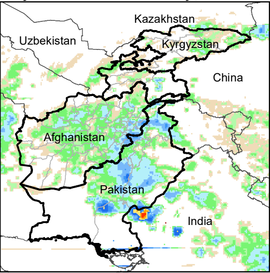
Daily Rainfall estimate for 1 May., 2005
