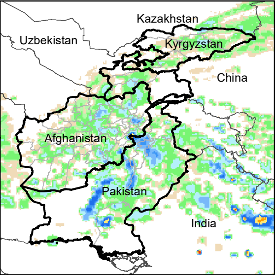
Daily Rainfall estimate for 5 May., 2005
