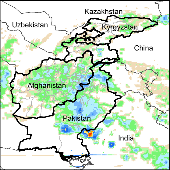
Daily Rainfall estimate for 4 May., 2005
