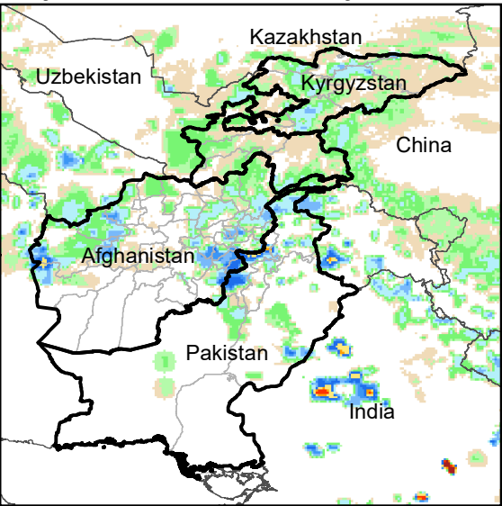
Daily Rainfall estimate for 7 May., 2005
