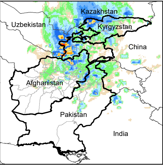
Daily Rainfall estimate for 8 May., 2005
