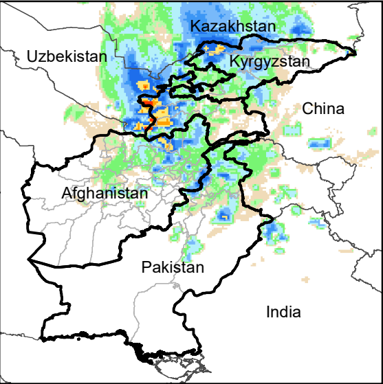
Daily Rainfall estimate for 11 May., 2005
