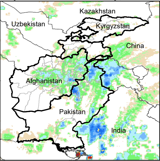
Daily Rainfall estimate for 29 May., 2005
