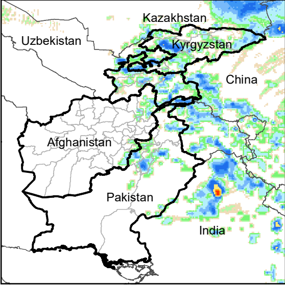
Daily Rainfall estimate for 6 Jun., 2005
