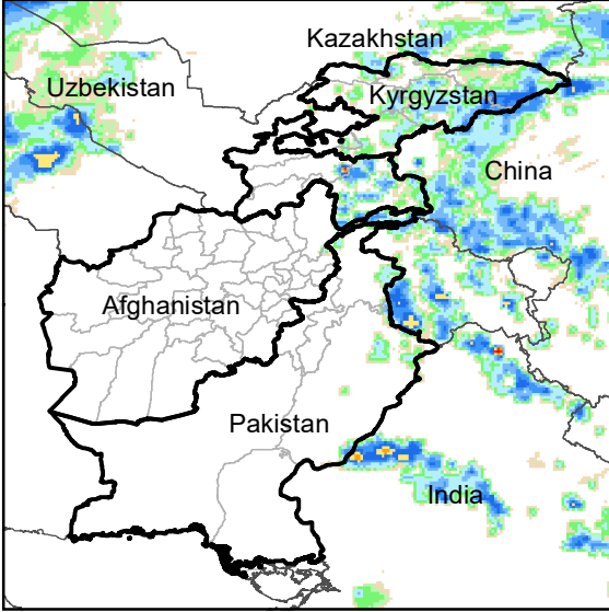
Daily Rainfall estimate for 7 Jun., 2005
