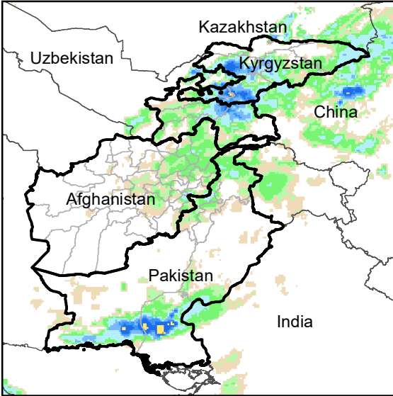
Daily Rainfall estimate for 15 Jun., 2005
