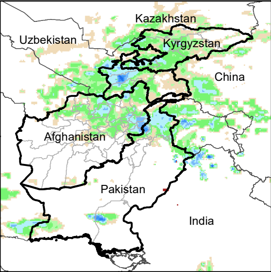
Daily Rainfall estimate for 13 Jun., 2005
