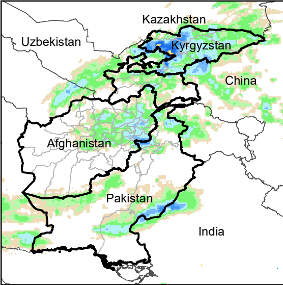
Daily Rainfall estimate for 14 Jun., 2005
