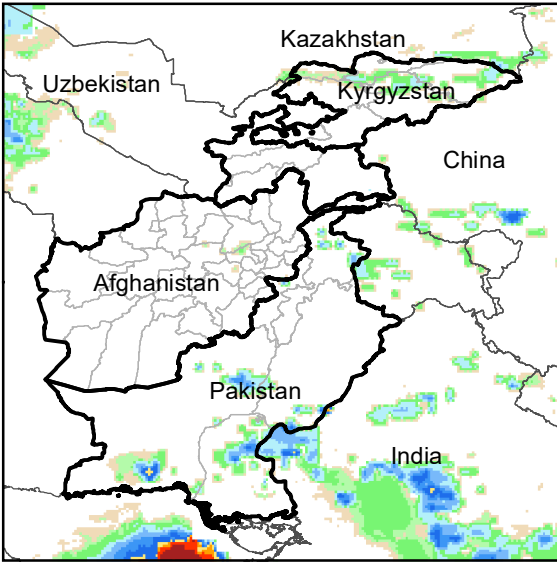
Daily Rainfall estimate for 21 Jun., 2005
