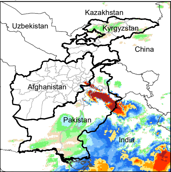
Daily Rainfall estimate for 5 Jul., 2005
