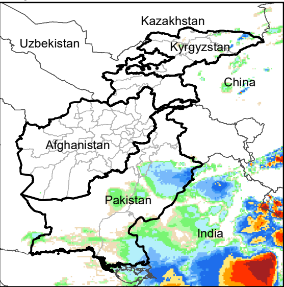
Daily Rainfall estimate for 6 Jul., 2005
